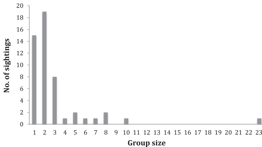
FIGURE 2 Number of sightings per group size of humpback dolphins ( Sousa plumbea ) observed in Algoa Bay between June 2008 and May 2011. Note: there were no sightings recorded with group sizes of 11–22 individuals
