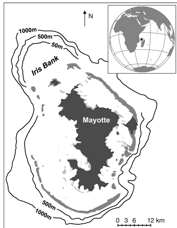
Fig. 1. The study area: Mayotte Island ( 12^\circ 50' \text{S} , 45^\circ 10' \text{E} ), Comoros archipelago
