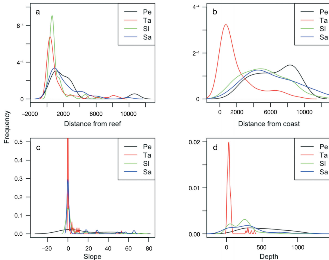
Fig. 3. Density plots of dolphin sightings around Mayotte in relation to physiographical variables: distance from (a) the nearest reefs (m) and (b) the coast (m); (c) slope ( ^{\circ} ); and (d) depth (m). Pe: Peponocephala electra ; Ta: Tursiops aduncus ; SI: Stenella longirostris ; Sa: S. attenuata
