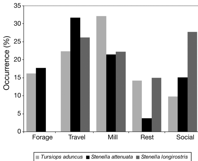
Fig. 5. Overall activity budgets for Indo-Pacific bottlenose dolphins, pantropical spotted dolphins and spinner dolphins around Mayotte, 2004–2009
