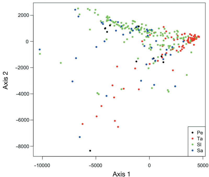
Fig. 4. Metric MDS plot of delphinid habitat in relation to physiographical variables. Pe: Peponocephala electra ; Ta: Tursiops aduncus ; SI: Stenella longirostris ; Sa: Stenella attenuata
