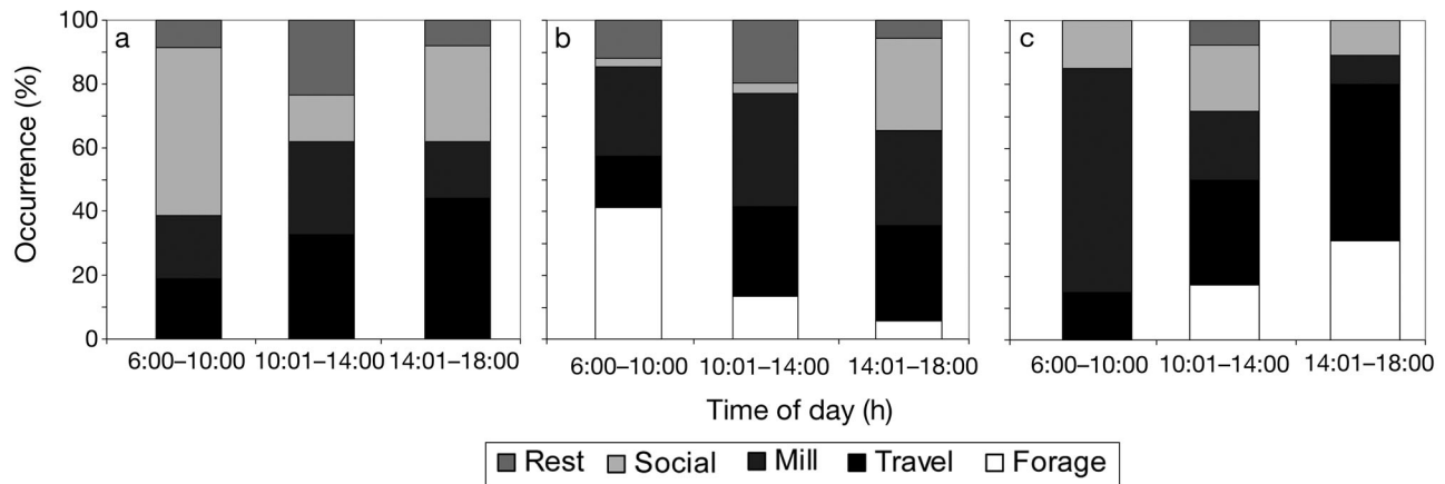
Fig. 6. Within day variations of behavioural budget in (a) spinner dolphin, (b) Indo-Pacific bottlenose dolphin and (c) pantropical spotted dolphin around Mayotte, 2004–2009
