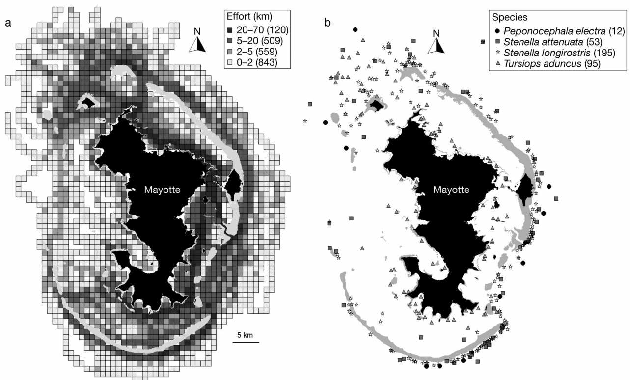
Fig. 2. Spatial distribution of (a) observation effort per 1 \text{ km}^2 cell and (b) dolphin sightings around Mayotte, Jul 2004–Apr 2009
